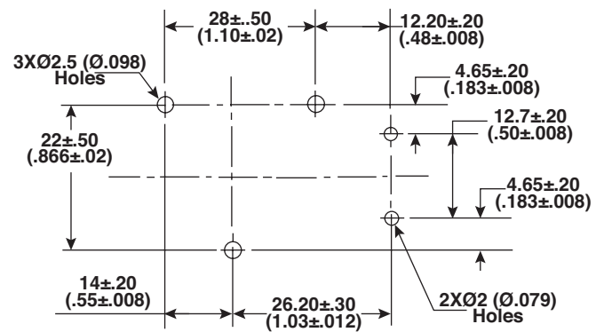
PCB Mounting Layout
